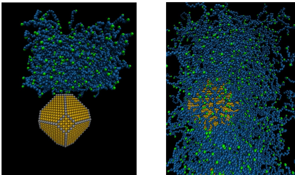
Figure 1: Snapshot from MD simulation of hybrid polyethylene/gold nanocomposite at 450K. Au nanoparticle ( 3101 atoms, diameter of 5.02 nm) and polyethylene (420 chains, 22-mers per chain) are shown. With yellow is the Au and with grey are the edges of Au nanoparticle. With blue are the CH 2 and with green the CH 3 monomers.
